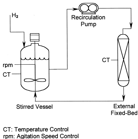
Fig. 1. Experimental set-up: recirculation system with an external fixed-bed reactor.
