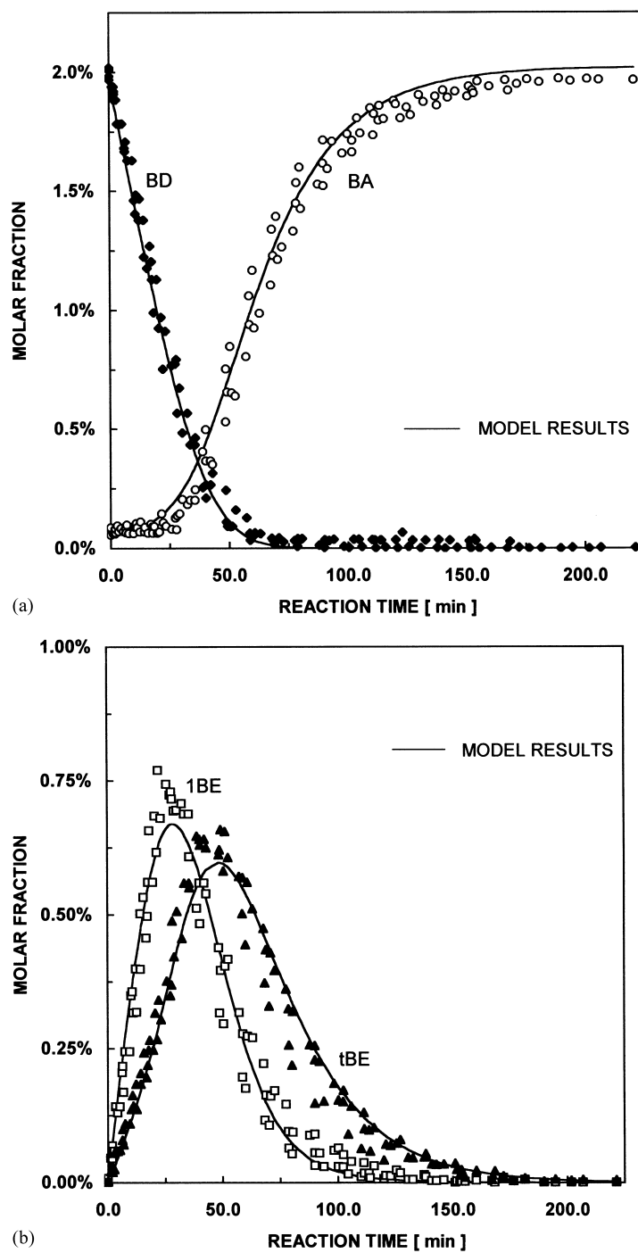
Fig. 4. Comparison between experimental and model predicted composition as a function of reaction time.
